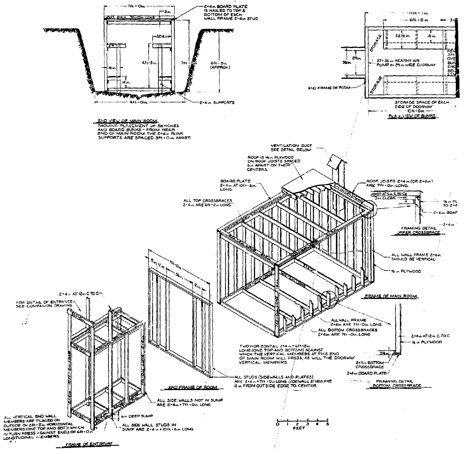
Figure A-15.1 Pictorial View of Lumber Version of Small-Pole Shelter
